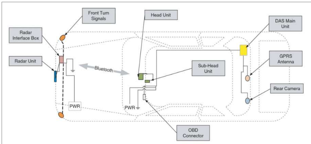
FIGURE 3 Data acquisition system schematic (Antin et al., 2015).
