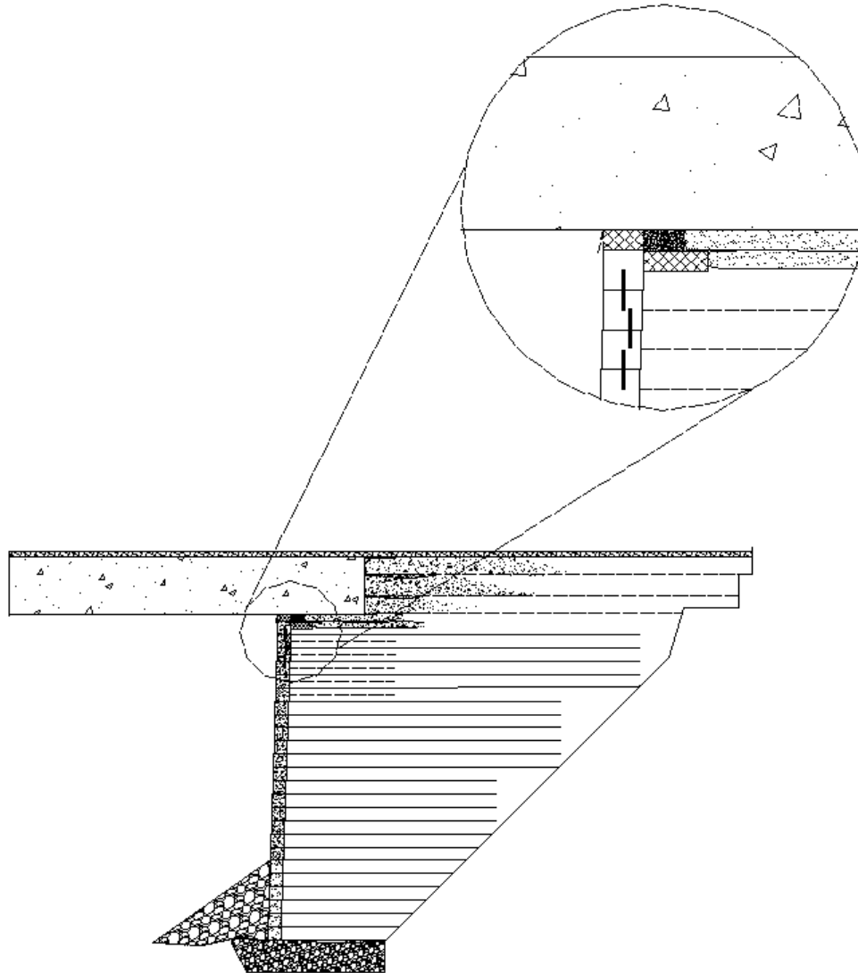
Figure 23. Illustration. Typical cross section of a GRS abutment face wall.
