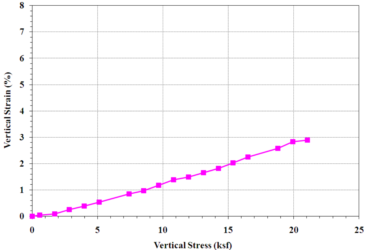
Figure 92. Graph. Vegas Mini-Pier stress-strain curve.
