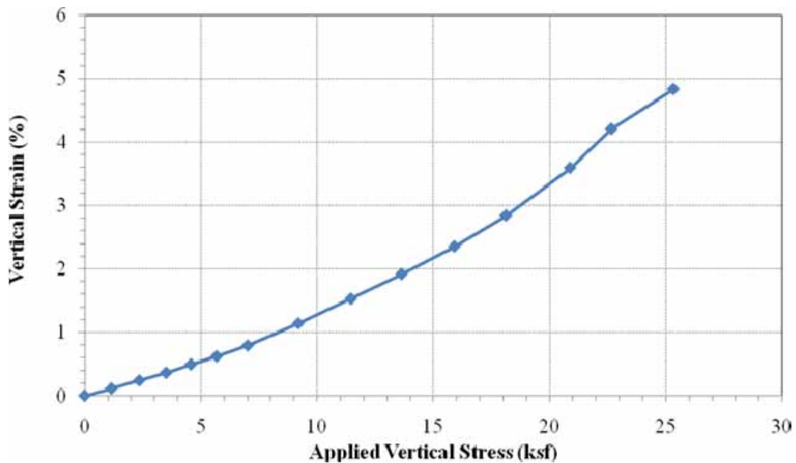
Figure 96. Graph. Defiance County stress-strain curve.
