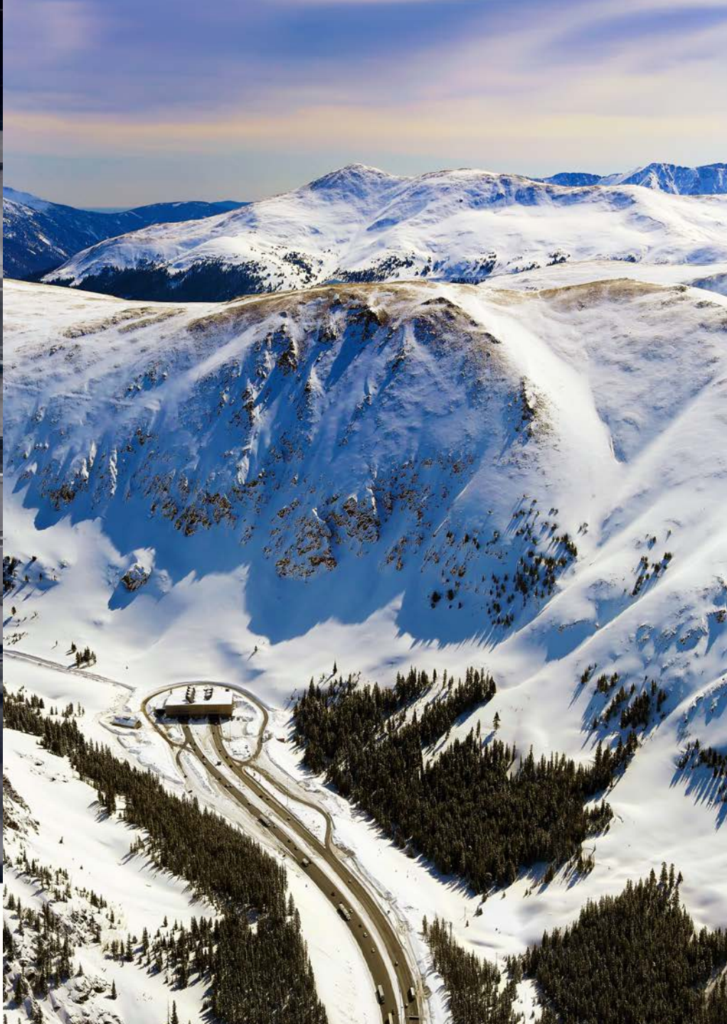
Roll YK Picture 11 (2:09 p.m.) West Tunnel, Station "View north showing progress of tile wall panel installation- T.D.T.
