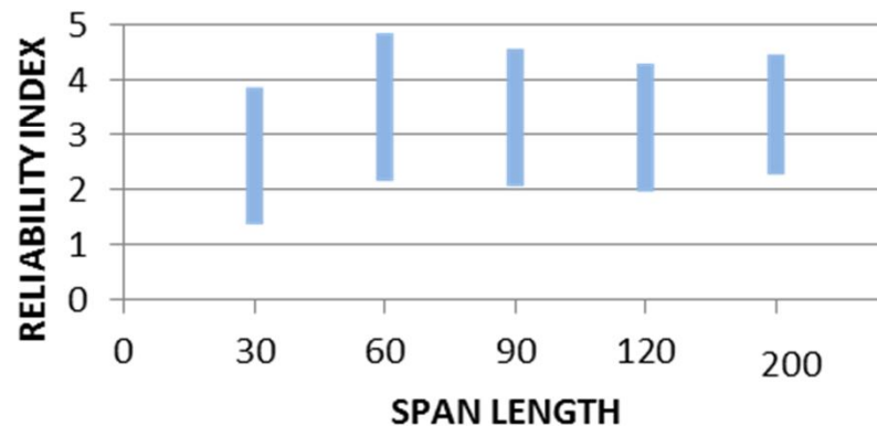
Reliability Indices AASHTO Standard Specifications
