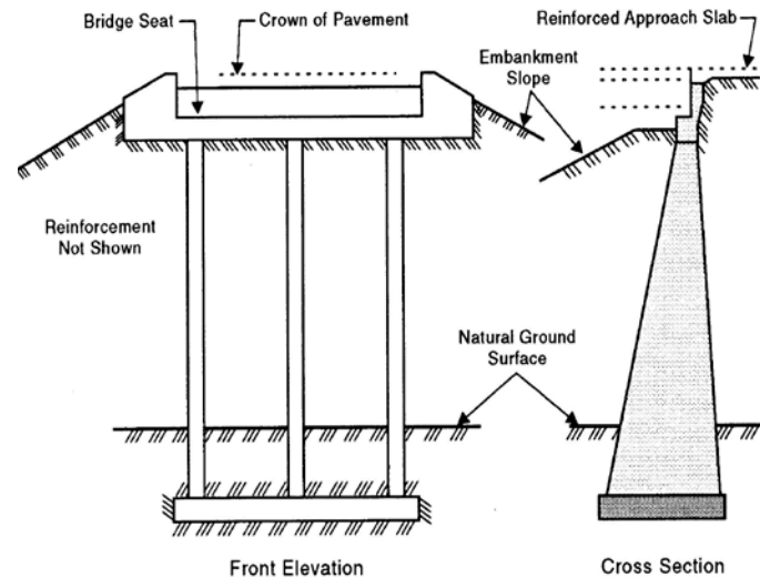
Typical Spill-Through Abutment
