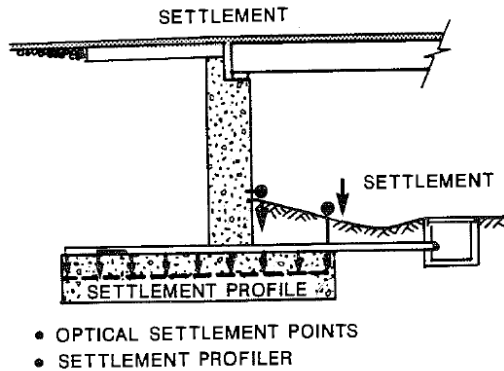
Figure 2. Settlement equipment for structures.
