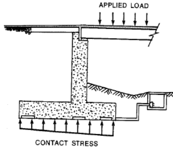
Figure 4 Contact stress and test loading.
