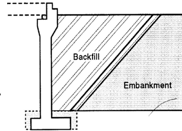
Typical Full-Height Closed or High Abutment
