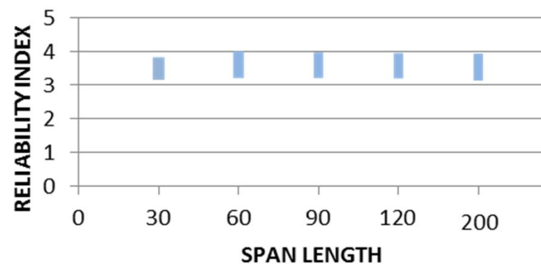
Reliability Indices AASHTO LRFD
