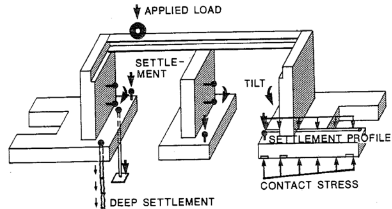
Figure 7. Conceptual plan: fully instrumented bridge.
