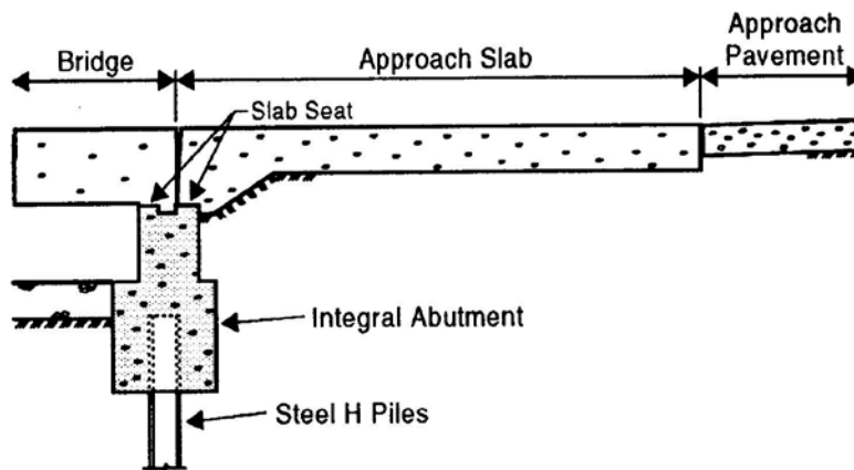
Typical Integral Abutment
