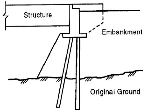
Typical Perched Abutment
