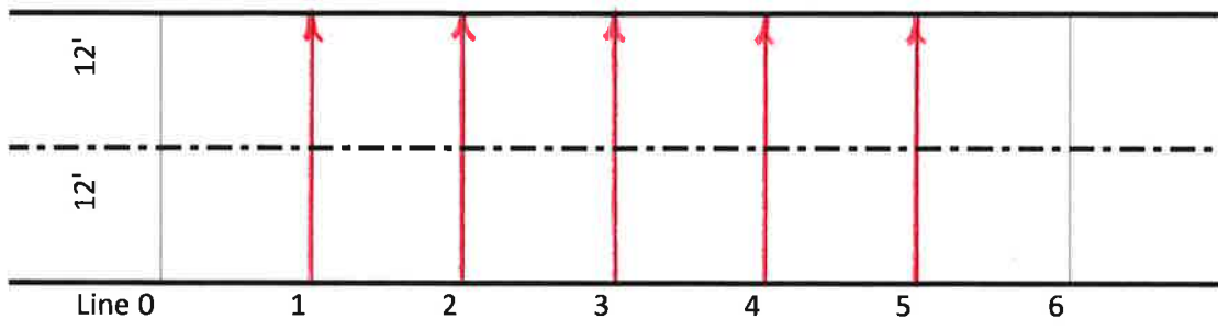
Plan for collecting Antenna Verification Data Center Antenna on Lines 1-5
